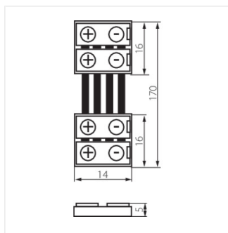
CONNECTOR RGB 10-CPC
