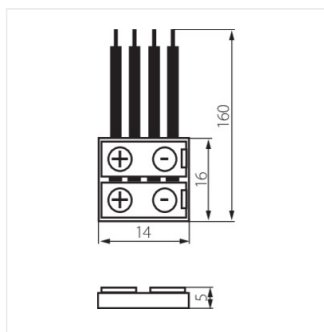
CONNECTOR RGB 10-CP
