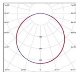
DAISY FENIX NG-R White 24W
