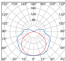
TRUST EVG PS 2 × 36W
