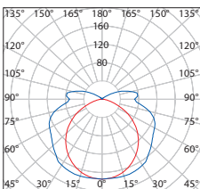
TRUST EVG PS 2 × 18W
