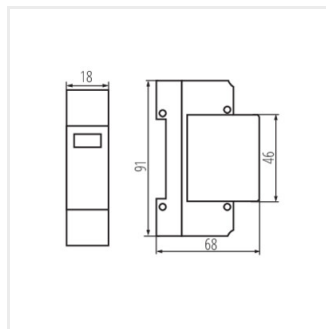
KSPD-T1T2 275/100 1PN
