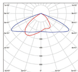
DAISY BOSTON PLUS 100W NW
