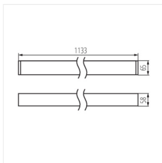
AL 23W-830-RST-W-NT
