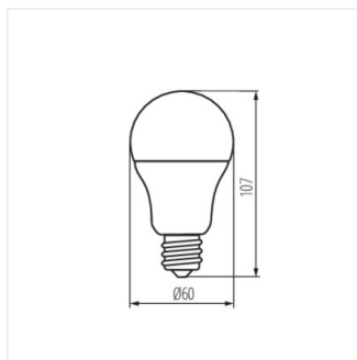
A60 N LED 8,5W E27
