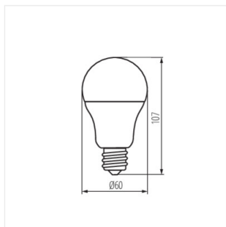
A60 N LED 5,5W E27
