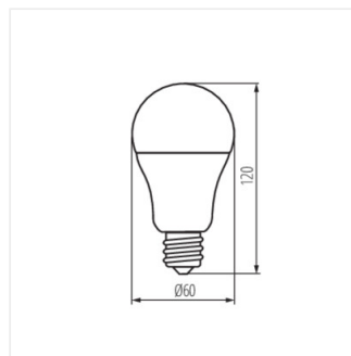
A60 N LED 14W E27
