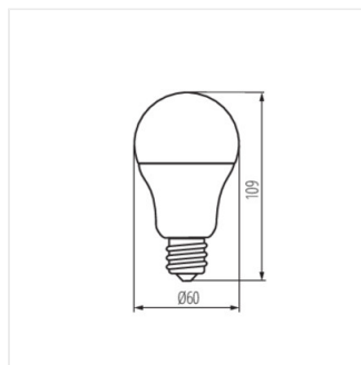
A60 N LED 10W E27
