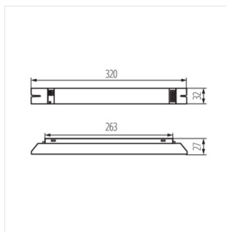
BLV2-158H-EVG
