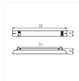
BLV2-3-4x14H-EVG
