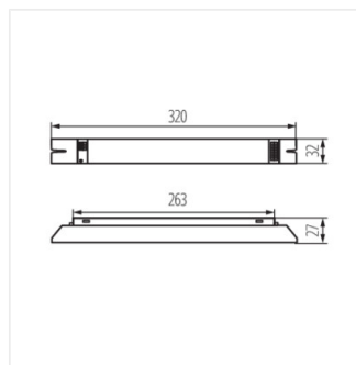
BLV2-236H-EVG
