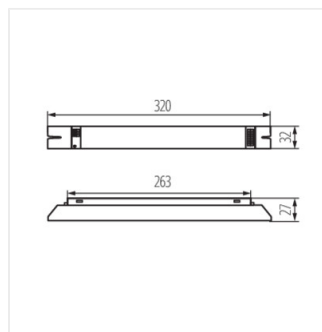
BLV2-258H-EVG
